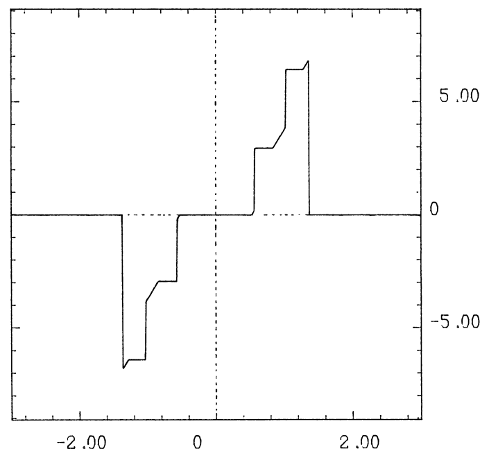
Figure 1. Stylized Sensitivity Curve of the LMS in One Dimension, Given by SC(x) = n(T_n(y_1, \dots, y_{n-1}, x) - T_{n-1}(y_1, \dots, y_{n-1})) , Where y_i = \Phi^{-1}(i/n) , for n = 10 .
